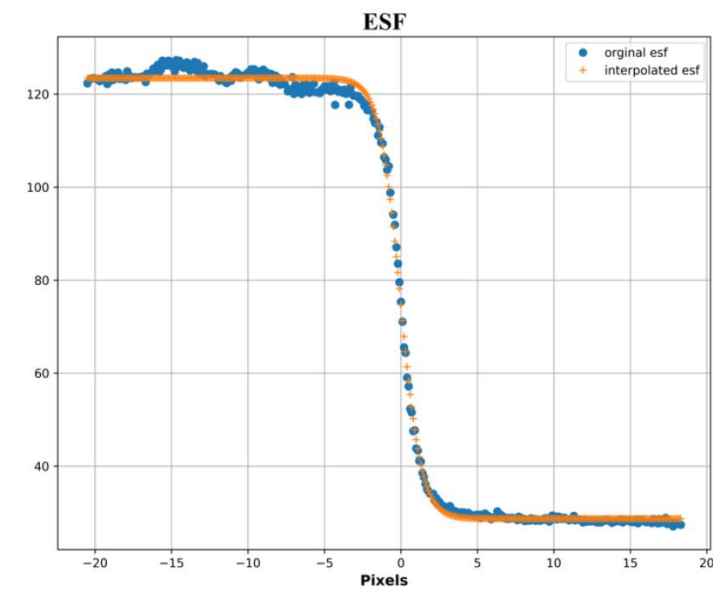
Figure 13 - ESF Interpolation.
