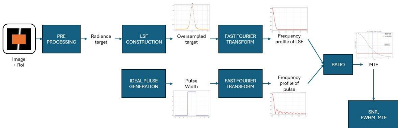
Figure 2 - IQ Toolset – MTF Bridge workflow.
