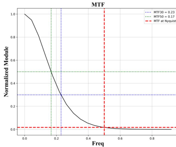
Figure 12 - MTF Validation.
