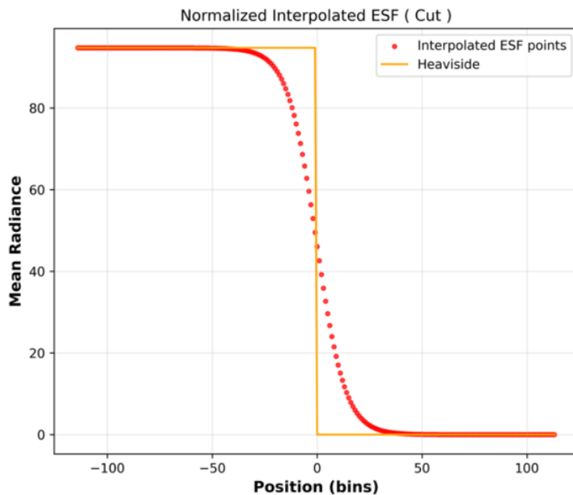
Figure 22 - Interpolated ESF.
